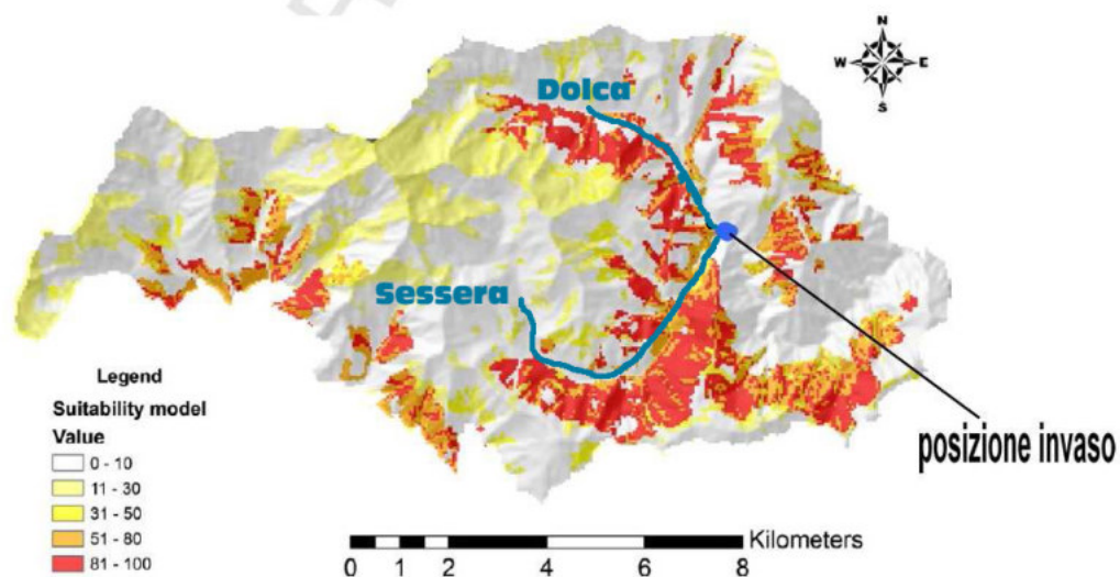
Fig. 5. A suitability map, based on GARP model, for the stenotopic species Carabus olympiae . Warmer colors represent increasing probability levels of presence. (For interpretation of the references to color in this figure legend, the reader is referred to the web version of this article.)
