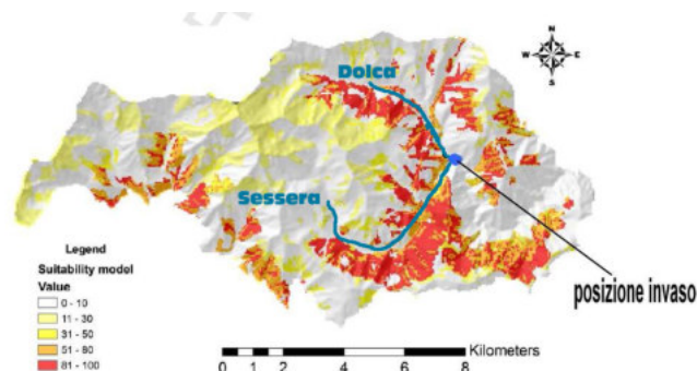
Fig. 5. A suitability map, based on GARP model, for the steno-endemic species Carabus olympiae . Warmer colors represent increasing probability levels of presence. (For interpretation of the references to color in this figure legend, the reader is referred to the web version of this article.)
